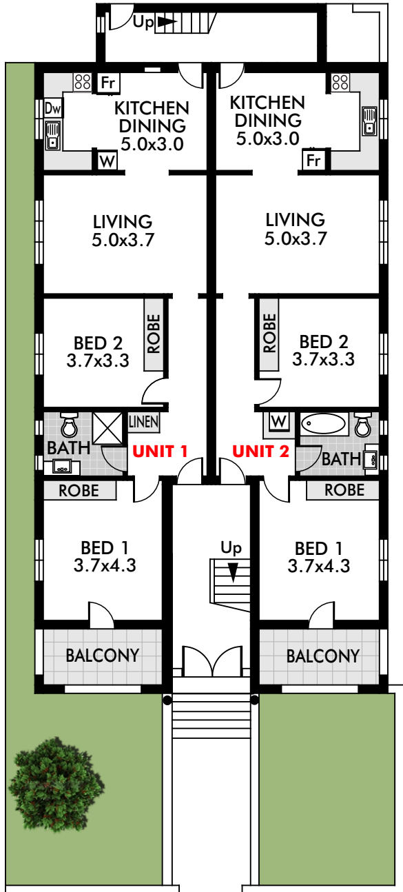
GROUND FLOOR
